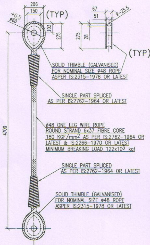
4 SETS SLING WITH THIMBLES AS DRAWN MKD.- (S-1) FOR HANGING DEVICE MKD: H-1
