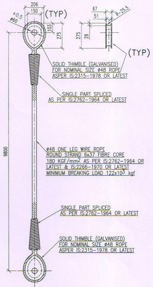
4 SETS SLING WITH THIMBLES AS DRAWN MKD.- (S-2) FOR HANGING DEVICE MKD: H-2
